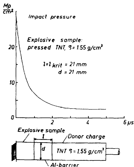
Fig 2 - Barrier test
